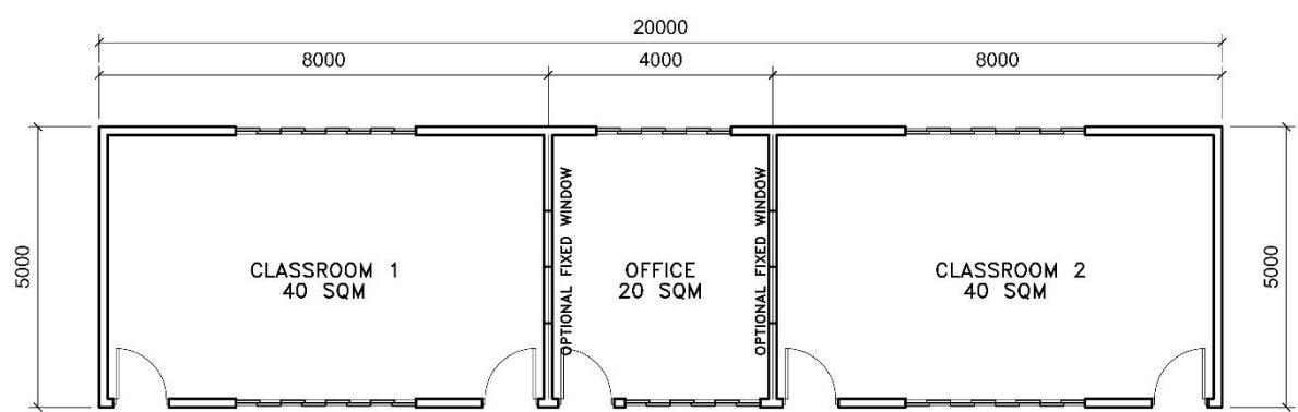
FLOOR PLAN (OPTION 2)
