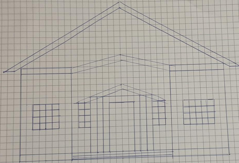
Front Elevation Multipurpose Hall- Magagu.
